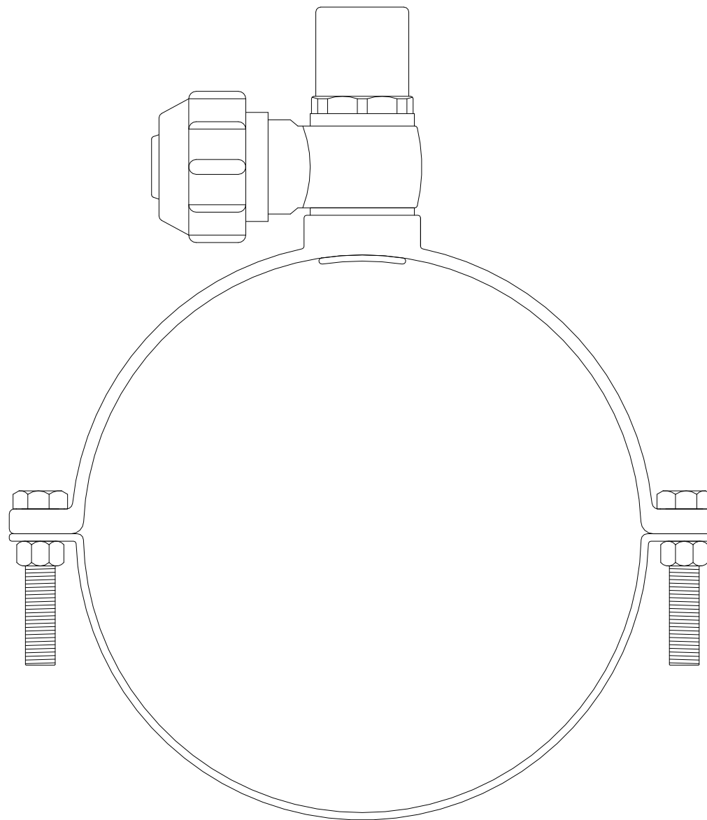
GPS PE PIPE SYSTEMS PROTECTA-LINE 32mm SELF-TAPPING FERRULE OFF-TAKE 225 x 32mm 44 762 424
