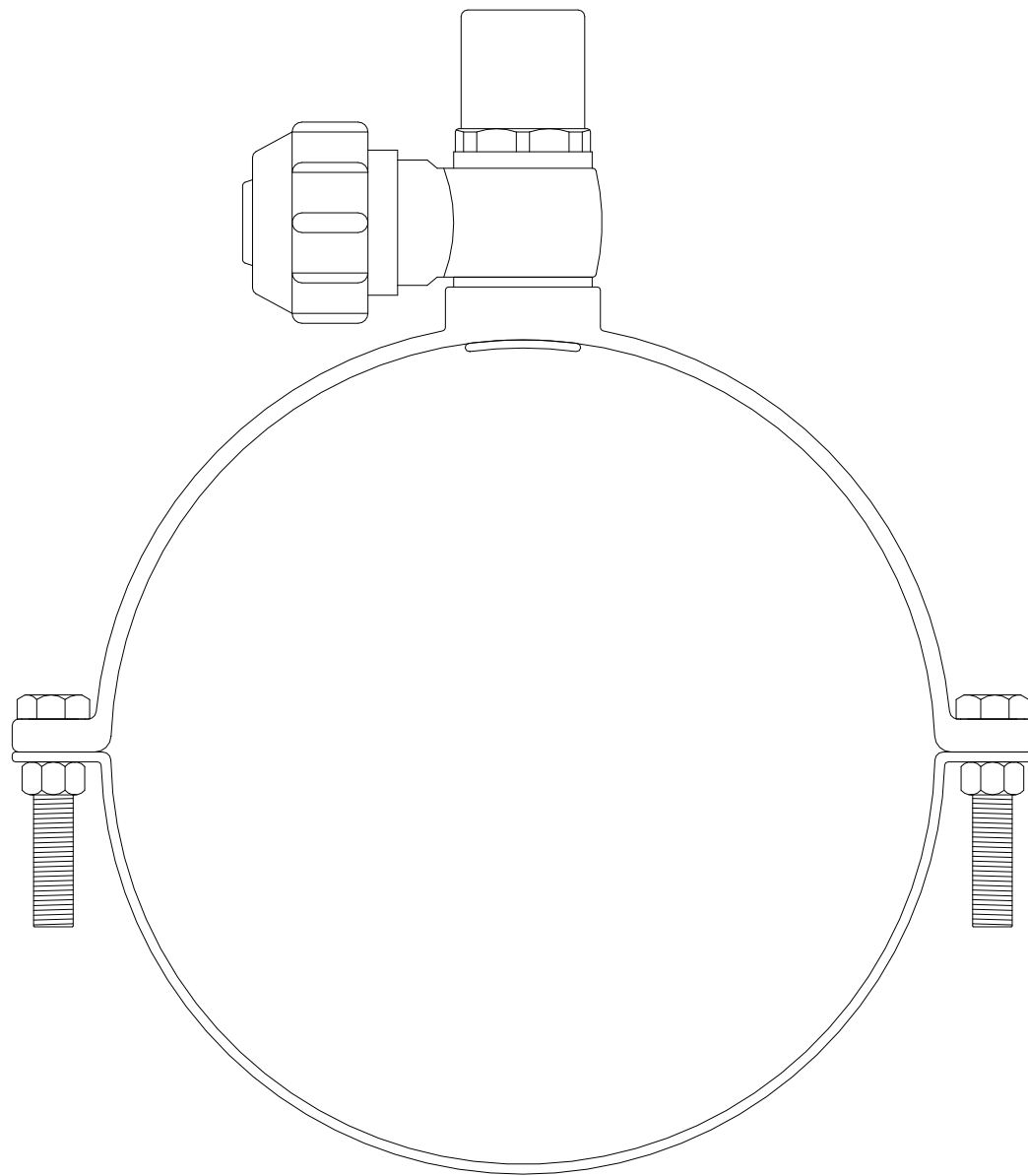
GPS PE PIPE SYSTEMS PROTECTA-LINE 32mm SELF-TAPPING FERRULE OFF-TAKE 250 x 32mm 44 762 425
