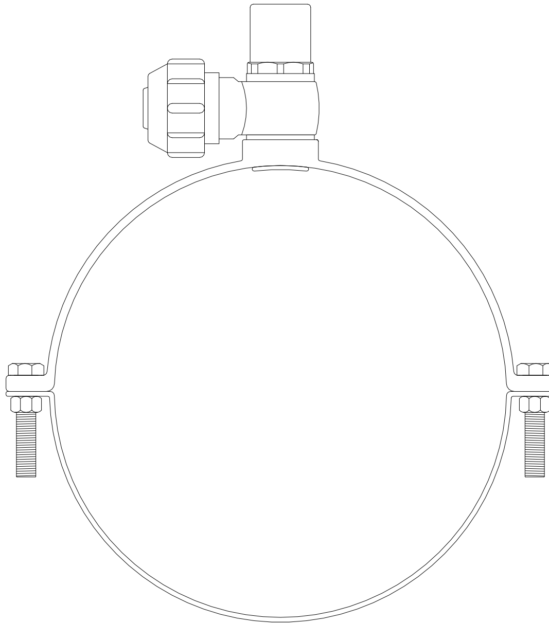
GPS PE PIPE SYSTEMS PROTECTA-LINE 32mm SELF-TAPPING FERRULE OFF-TAKE 280 x 32mm 44 762 426
