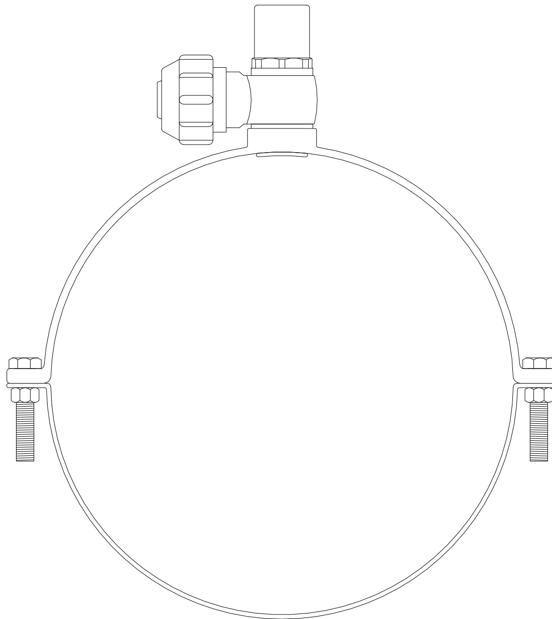
GPS PE PIPE SYSTEMS PROTECTA-LINE 32mm SELF-TAPPING FERRULE OFF-TAKE 315 x 32mm 44 762 427
