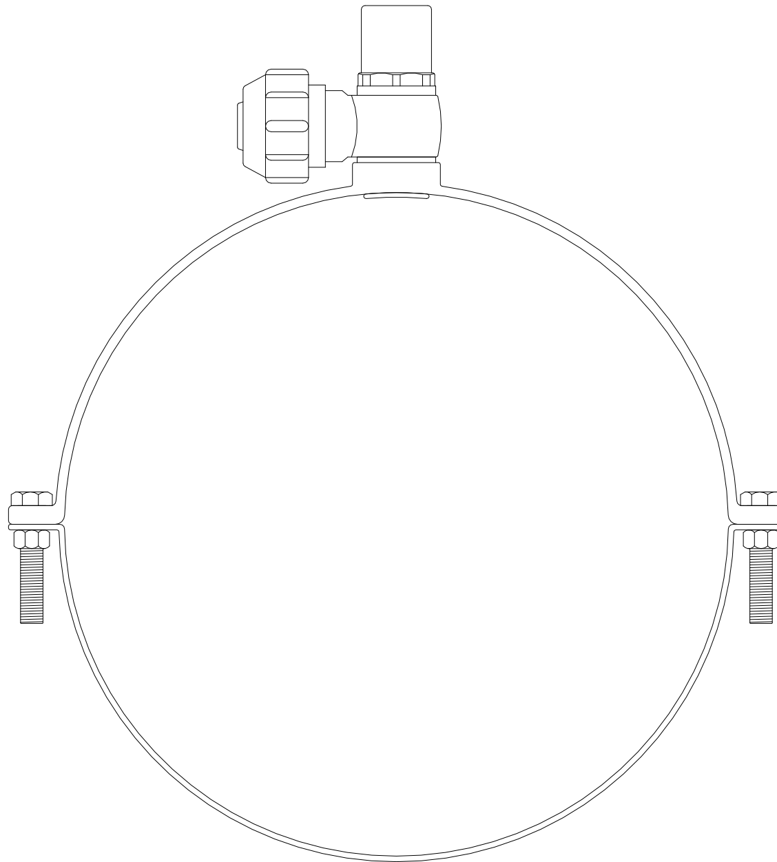
GPS PE PIPE SYSTEMS PROTECTA-LINE 32mm SELF-TAPPING FERRULE OFF-TAKE 355 x 32mm 44 762 428
