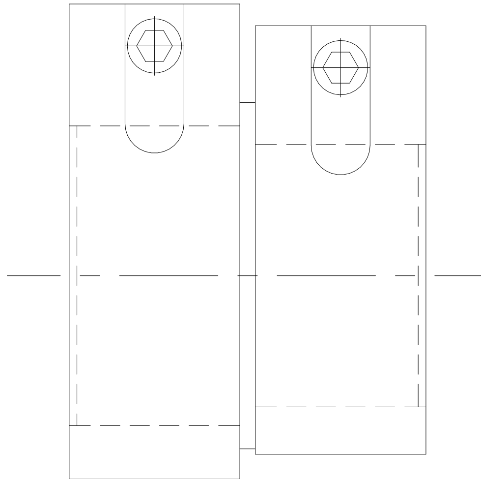
GPS PE PIPE SYSTEMS PROTECTA-LINE MECHANICAL FITTINGS REDUCER / 125 x 110mm (Supplied as a set with 2 half shells) PM 440 493
