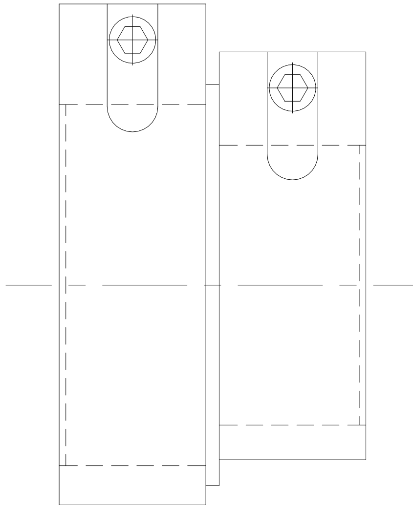
GPS PE PIPE SYSTEMS PROTECTA-LINE MECHANICAL FITTINGS REDUCER / 160 x 125mm (Supplied as a set with 2 half shells) PM 440 504
