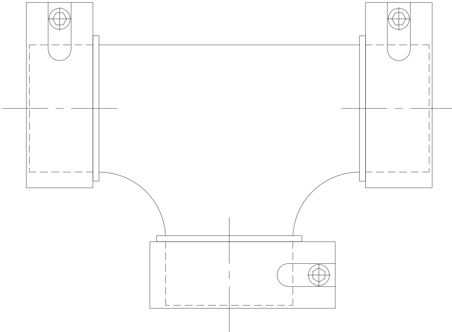
GPS PE PIPE SYSTEMS PROTECTA-LINE MECHANICAL FITTINGS EQUAL TEE / 125mm (Supplied as a set with 3 half shells) PM 220 315
