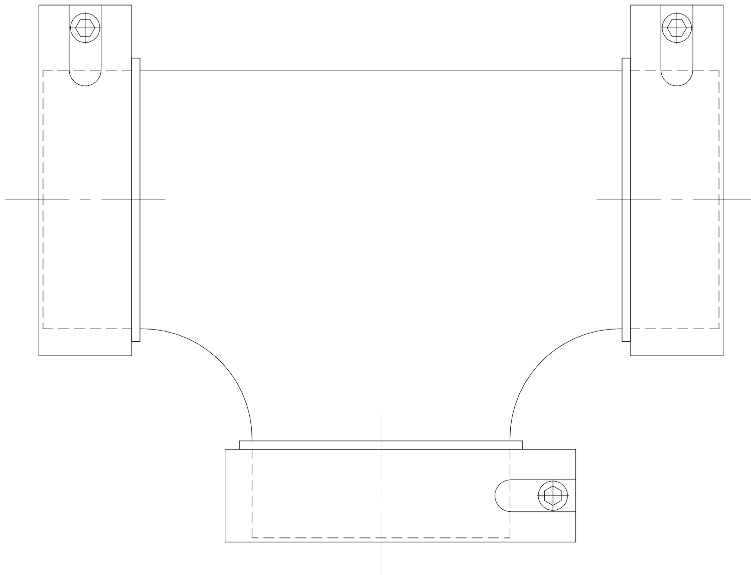
GPS PE PIPE SYSTEMS PROTECTA-LINE MECHANICAL FITTINGS EQUAL TEE / 180mm (Supplied as a set with 3 half shells) PM 220 318
